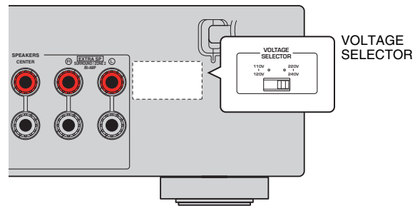
The unit (rear)
