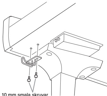
4 × 10 mm smala skruvar
