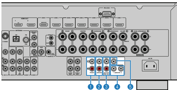
Receiver (baksida)
