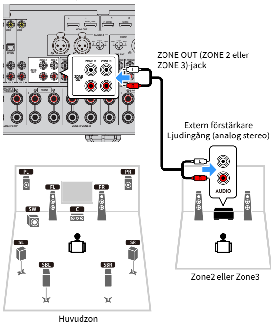
Receivern (baksida)
