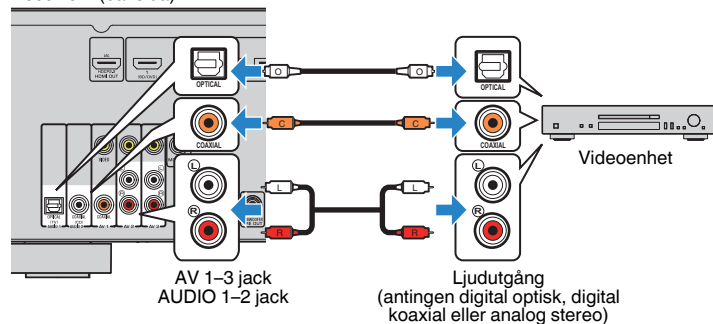
Receiveern (baksida)
