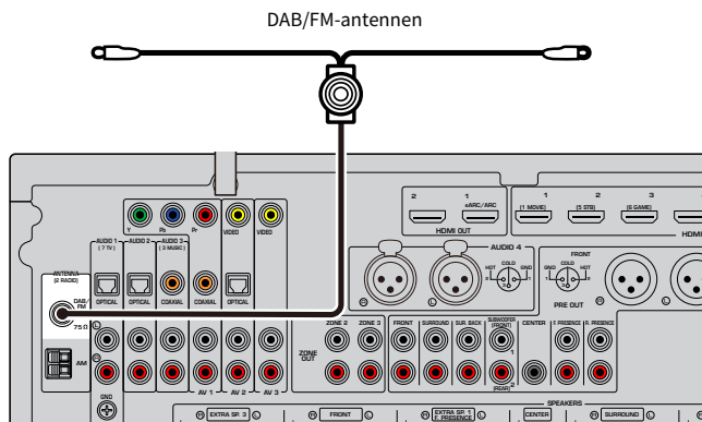
Receiver (baksida)
